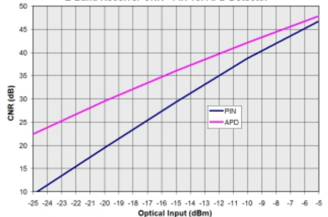
Advanced L-Band Rx CNR with PIN & APD
