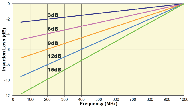
Figure 3 - Characteristics of Various Equalizers
