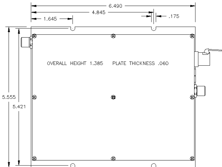
Figure 1 - OTOT-1000C-FF Mounting Diagram
